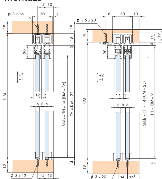
L - 3500 mm 67-E053.3248.350
